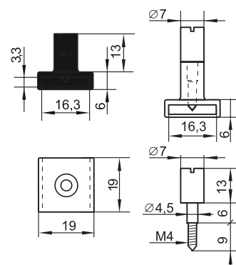
Prolongation Screw 13 mm
