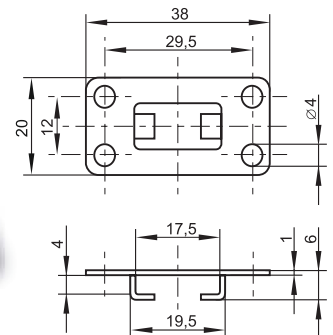
No. # 14.04.091 - 0,30 евро Metal Bar Guide holder for locking bars
