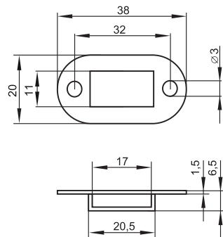
No. # 14.04.091 - 0,30 евро Metal Bar Guide holder for locking bars
