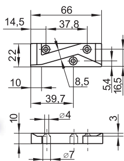
Antitilt Block Plastic Black Model 1018.030 No. # 14.03.271 Left Hand - 2.00 евро
