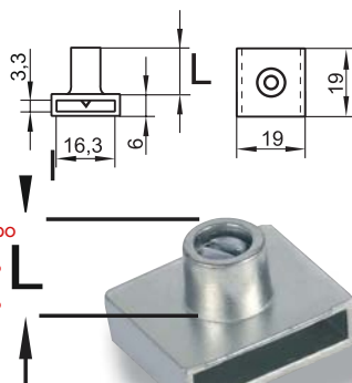
Prolongation Screw 13 mm
